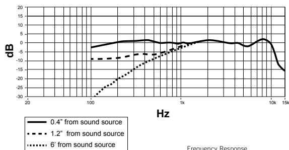
Frequency Response
